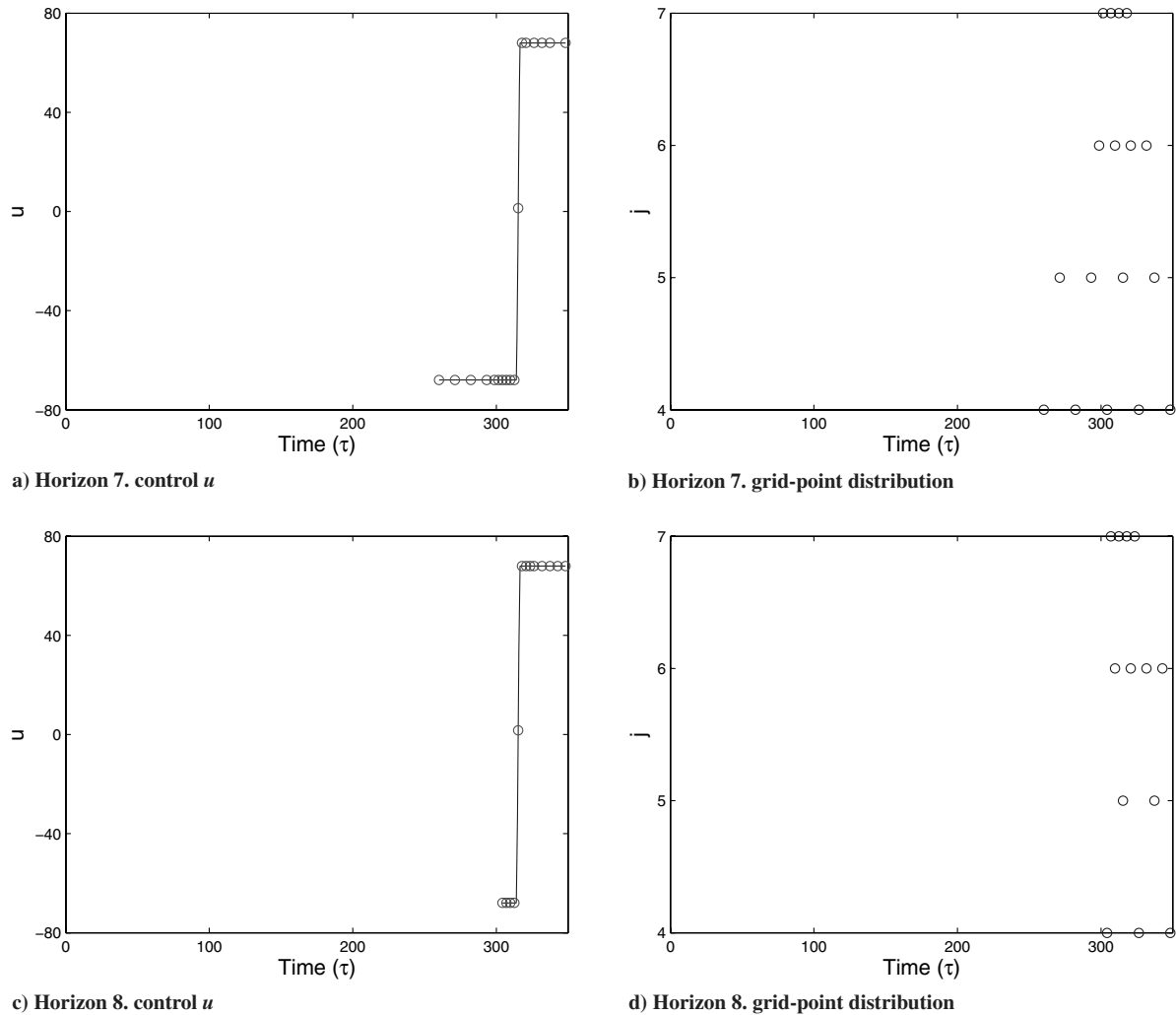
Fig. 7 Example 2: control time-history and grid-point distributions for horizons 7 and 8.
