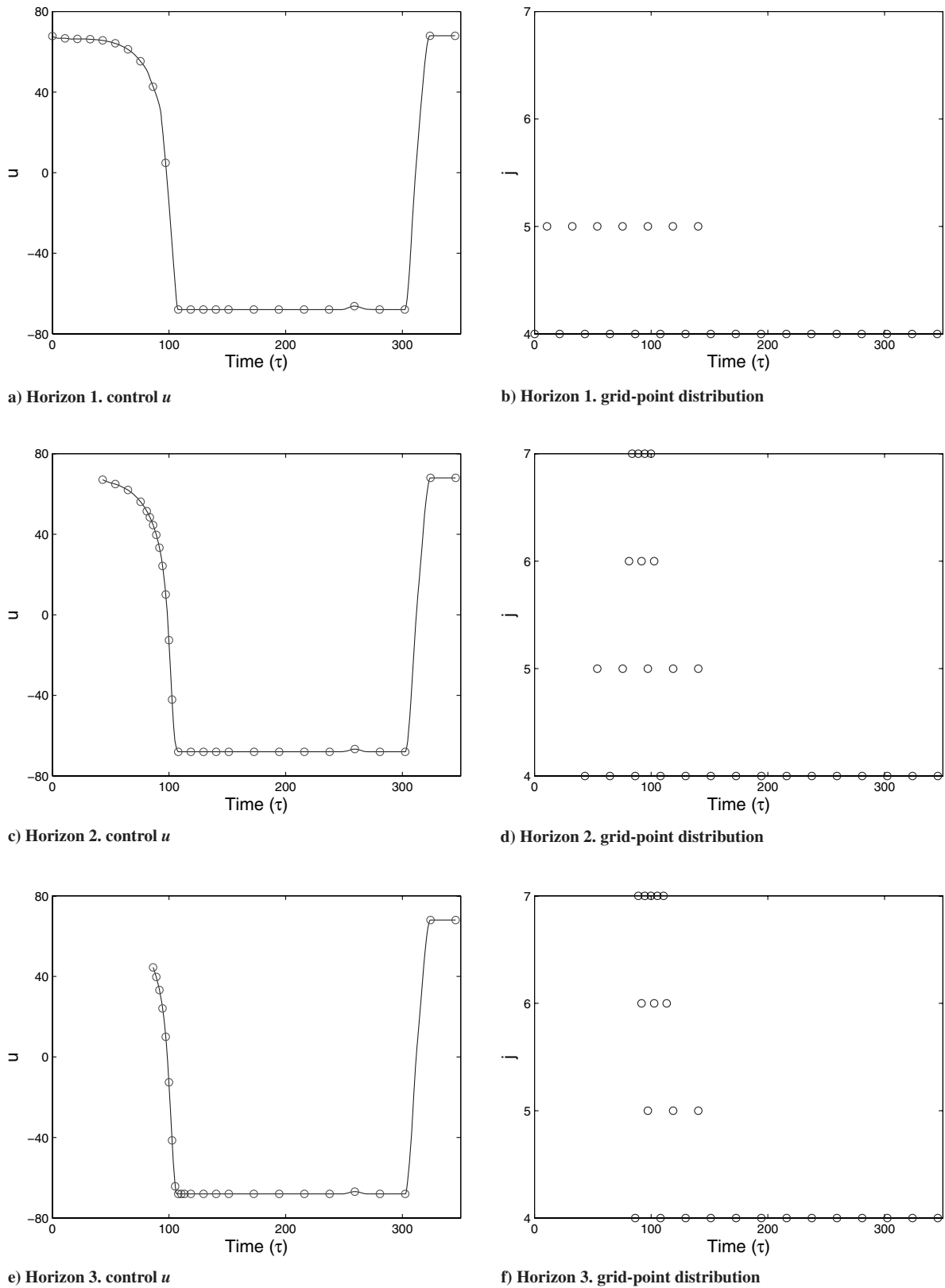
Fig. 5 Example 2: control time-history and grid-point distributions for horizons 1, 2, and 3.
